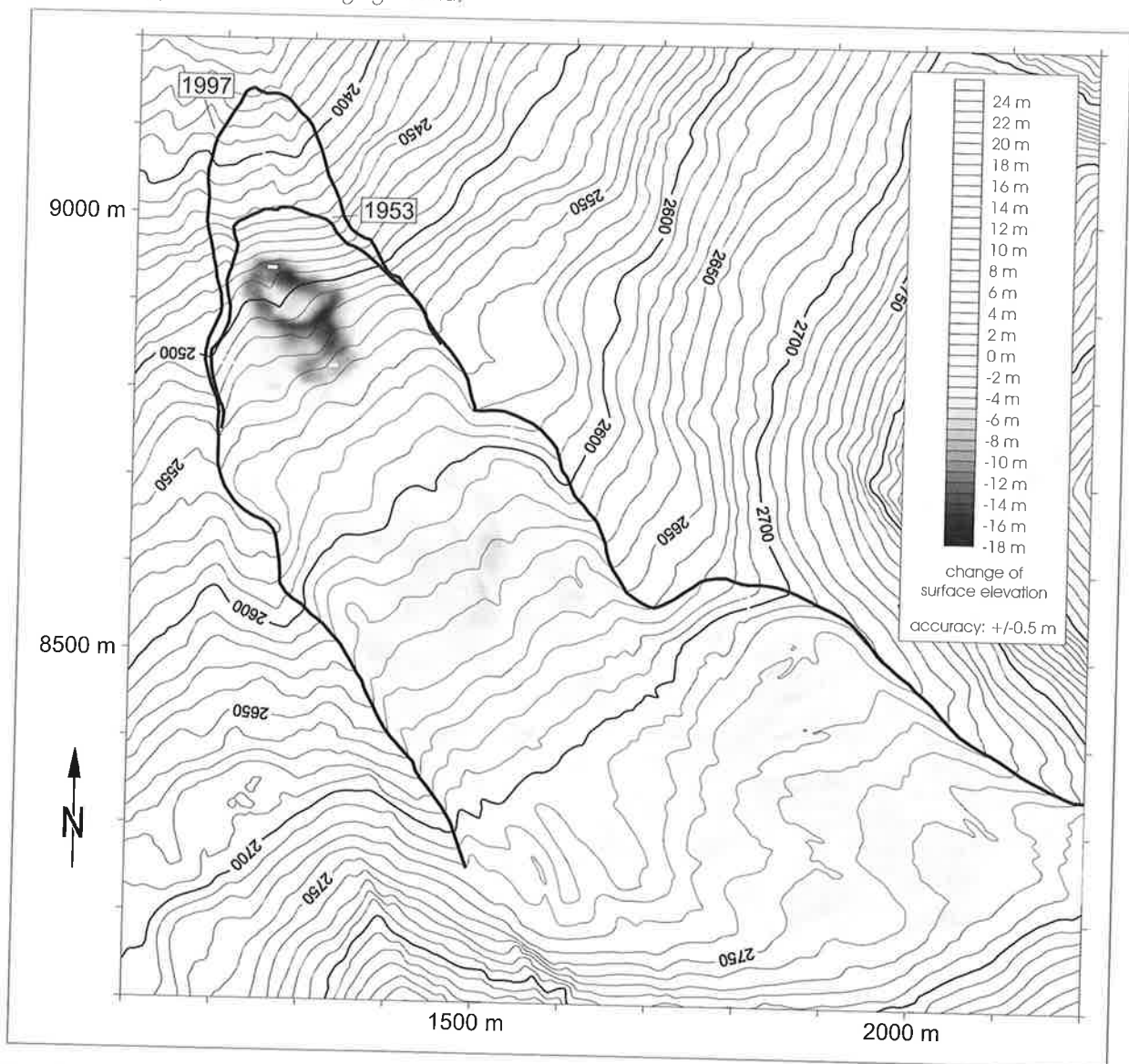
Figure 10: Change of surface elevation at Outer Hohebenkar rock glacier for the time period 1953-1997.
