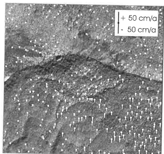
Figure 5f: Vertical component of the flow vectors 1953-1969, accuracy: \pm 2.5 \text{ cm a}^{-1} .
