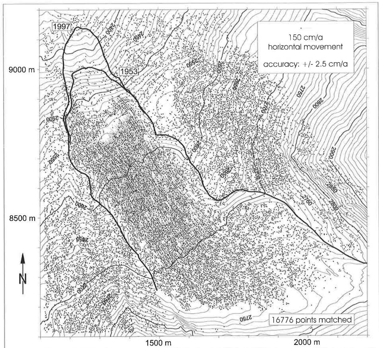
Figure 6: Flow vector field at Outer Hochebenkar rock glacier for the time period 1971-1977.
