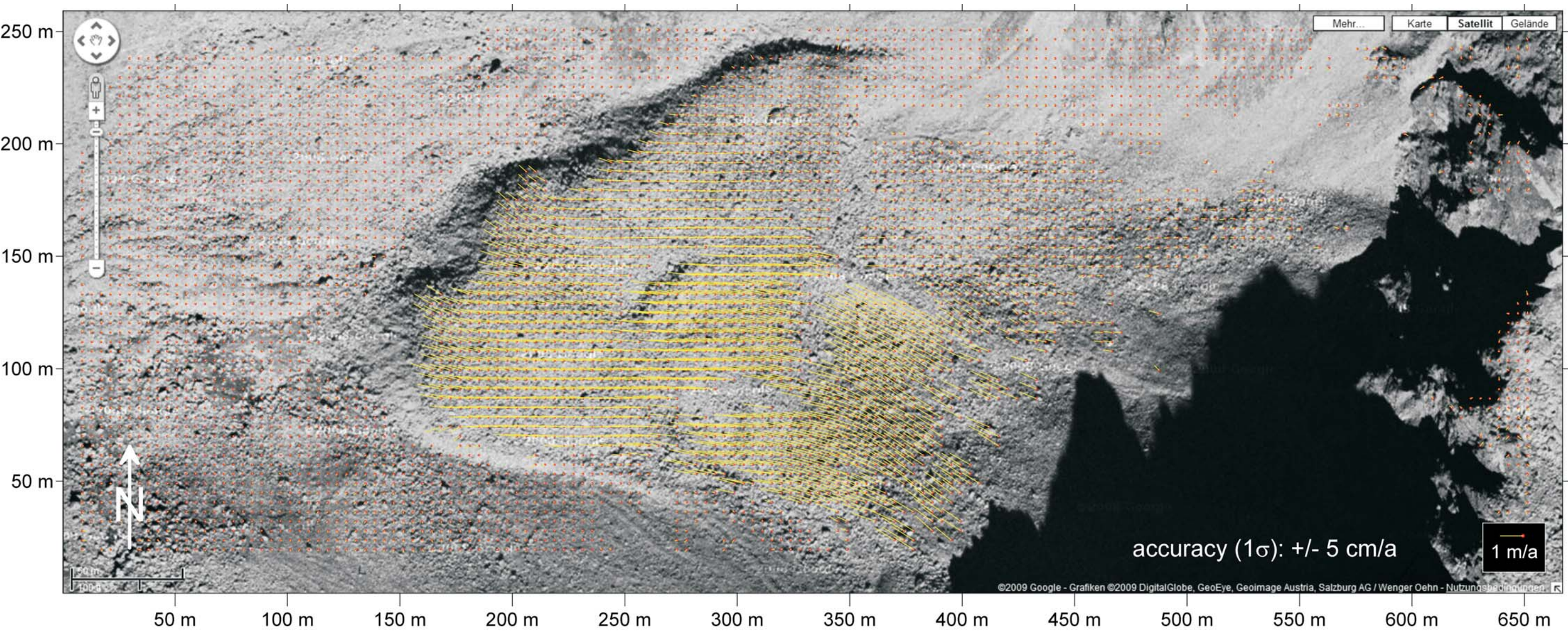
Vector field of mean annual horizontal movement (2002-2006) 5039 points by area-based image matching Method: NCC, r minimum 0.4 Template size: 25 x 25, max. back-matching distance: 1 pixel Grid spacing: 12 x 12
