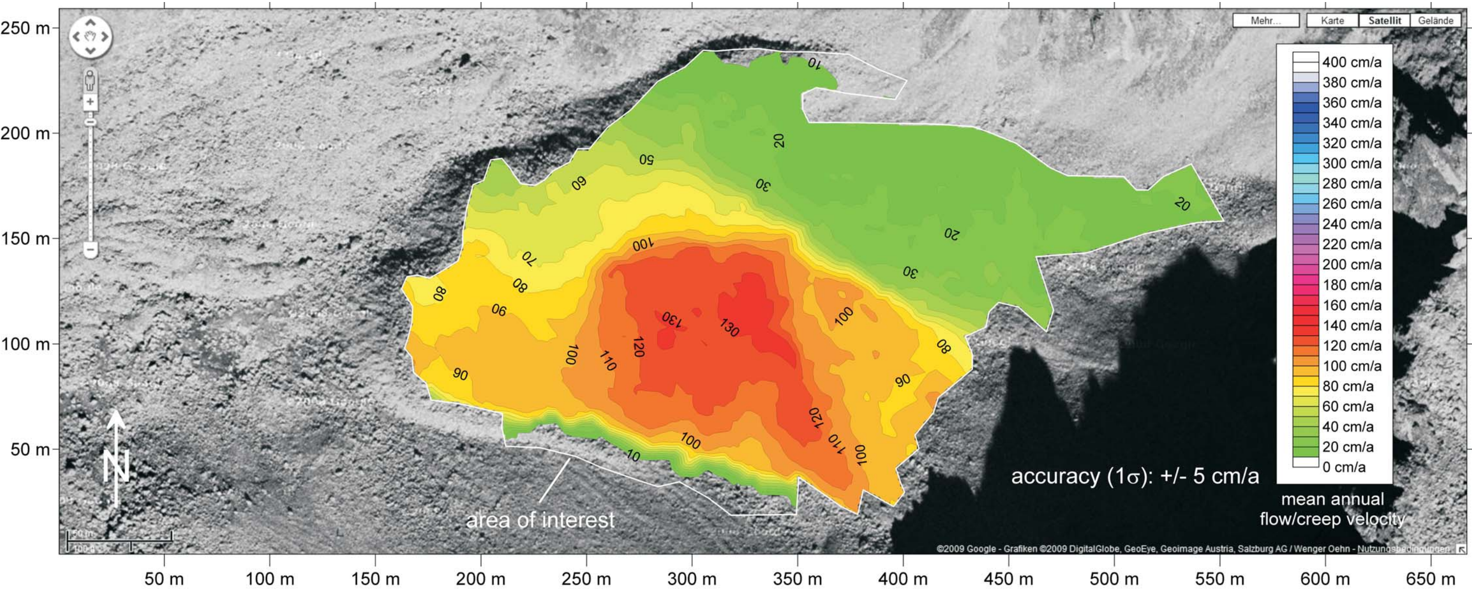
Isotachs of mean annual horizontal movement (2002-2006)
