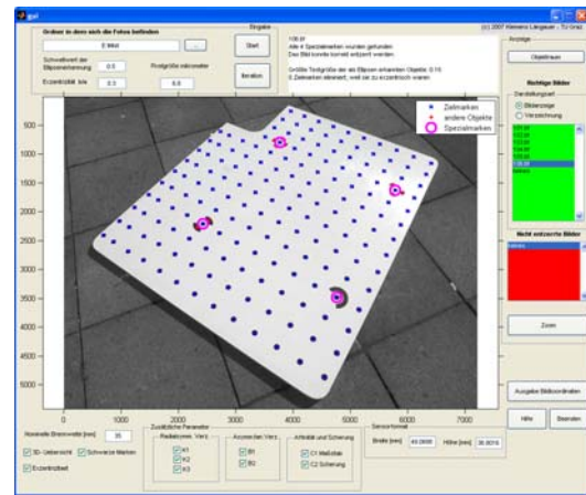
Figure 7. MATLAB tool for automated 2D measurements
