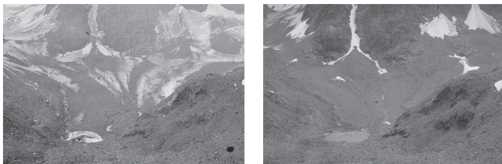
Figure 12: Terrestrial view of the central part of the Gössnitzkees Glacier. Left: a photo from 7 September 1988 taken with a Zeiss TAL photo-theodolite (photo: Robert Kostka and Viktor Kaufmann). Right: a photo from 20 August 2010 taken with a Nikon D300 digital camera. The photo at right also shows the glacial lake. The photos were taken from the same reference camera station (photo: Viktor Kaufmann).
