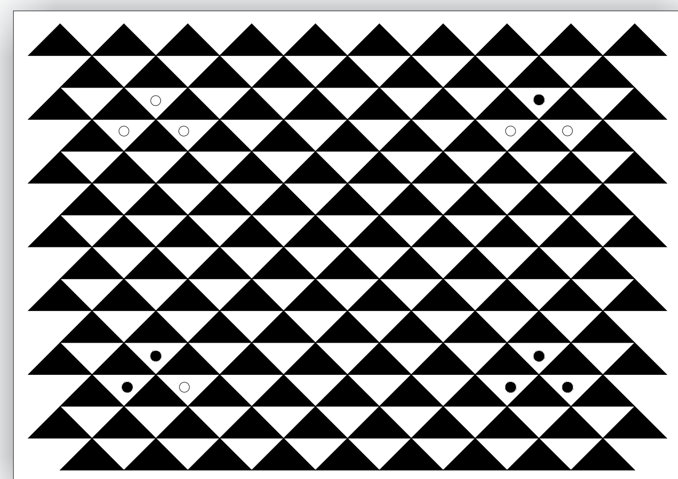
Planar calibration field of PhotoModeler 4.0
