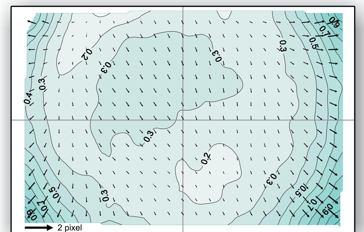
Interpolated displacement vectors: B channel
